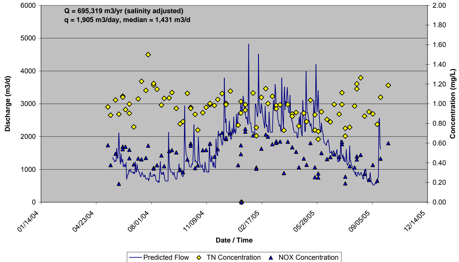
Figure IV-10. Discharge from Un-named Creek (solid blue line), nitrate+nitrite (blue symbols) and total nitrogen (yellow symbols) concentrations for determination of annual volumetric discharge and nitrogen load from the upper watershed to the head of Allen Harbor (Table IV-6).
