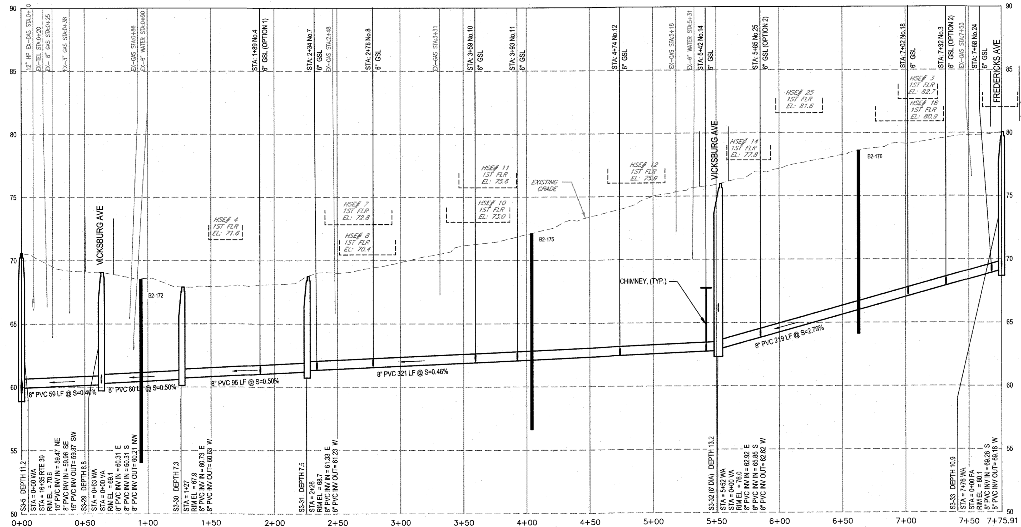
WILLIAMSBURG AVENUE - PROFILE SCALE HORIZ 1" = 40' VERT 1" = 4'
