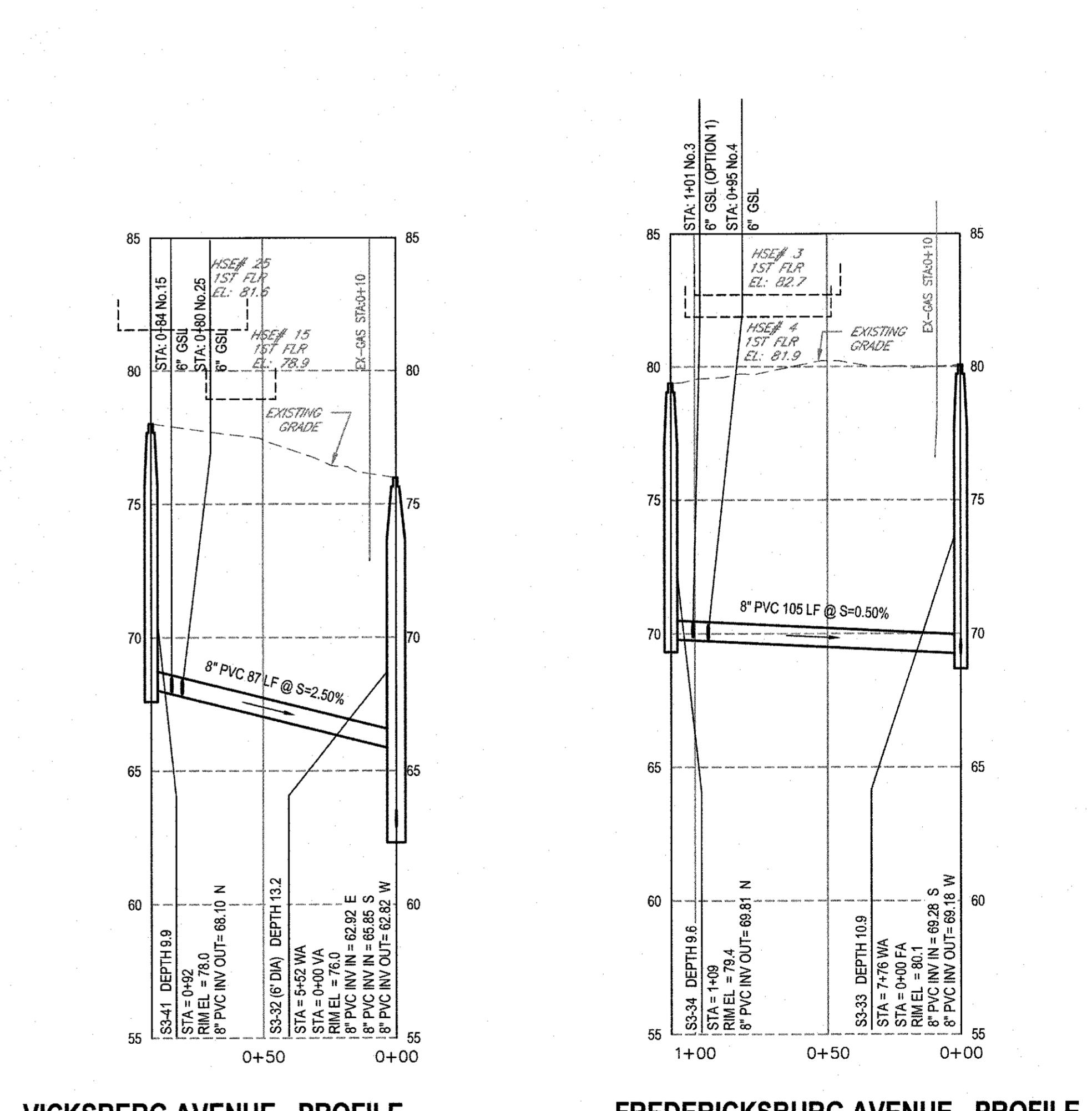
VICKSBURG AVENUE - PROFILE SCALE HORIZ 1" = 40' VERT 1" = 4'
