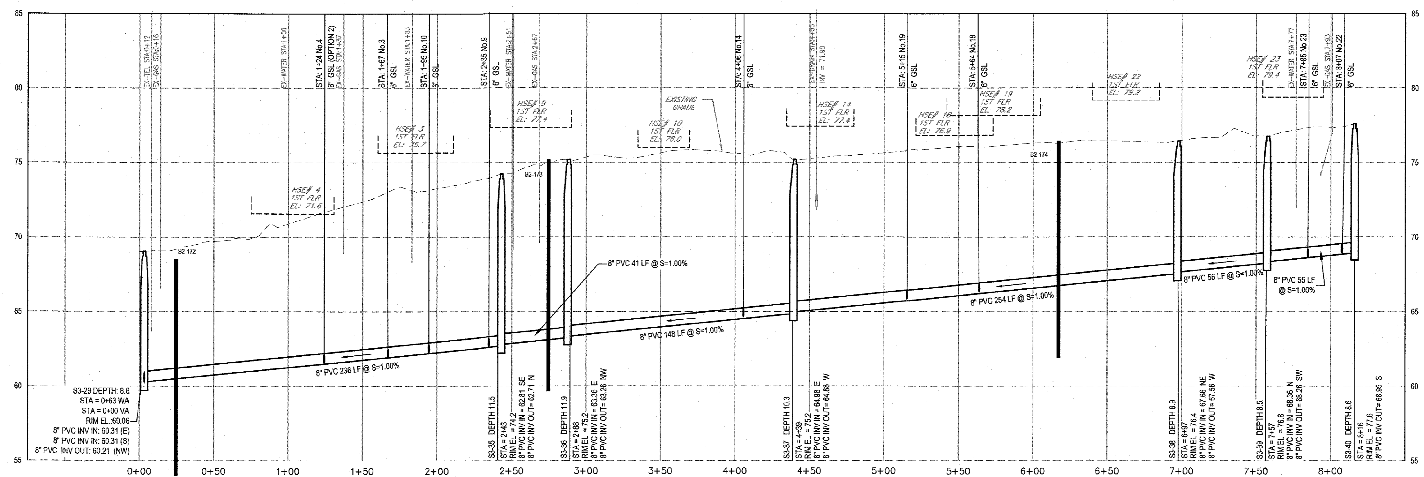
VICKSBURG AVENUE - PROFILE SCALE HORIZ 1" = 40' VERT 1" = 4'
