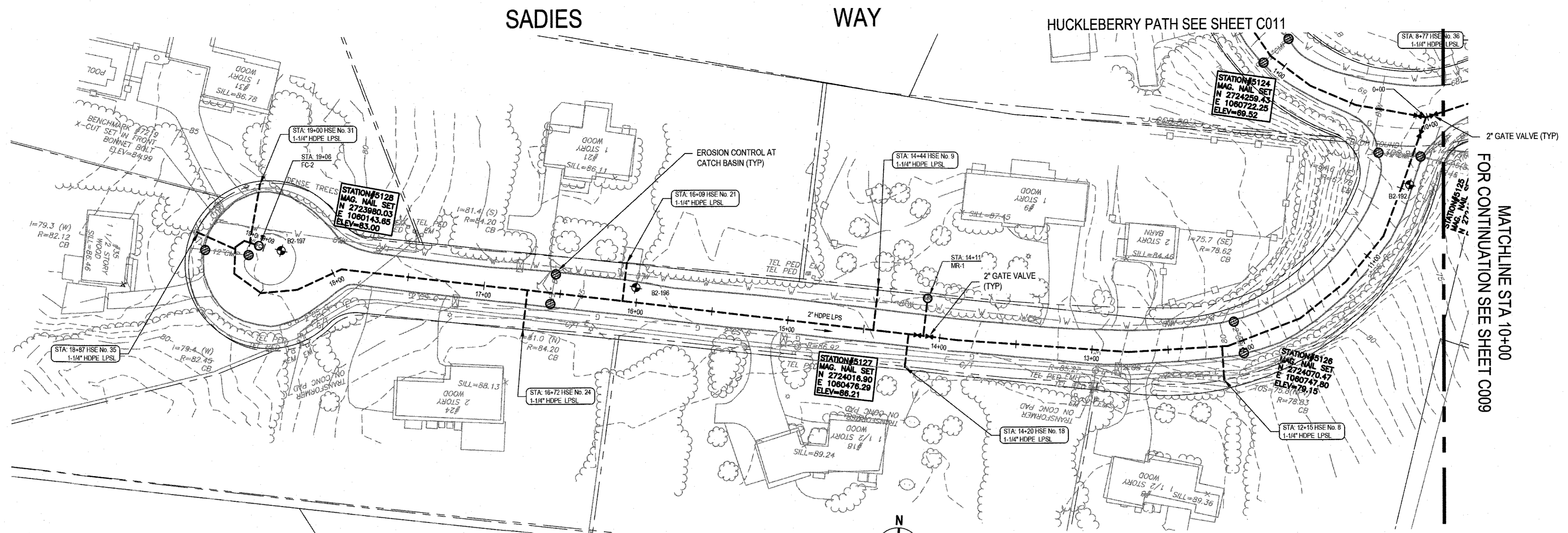
SADIES WAY - PLAN (BID ALTERNATE #3)
