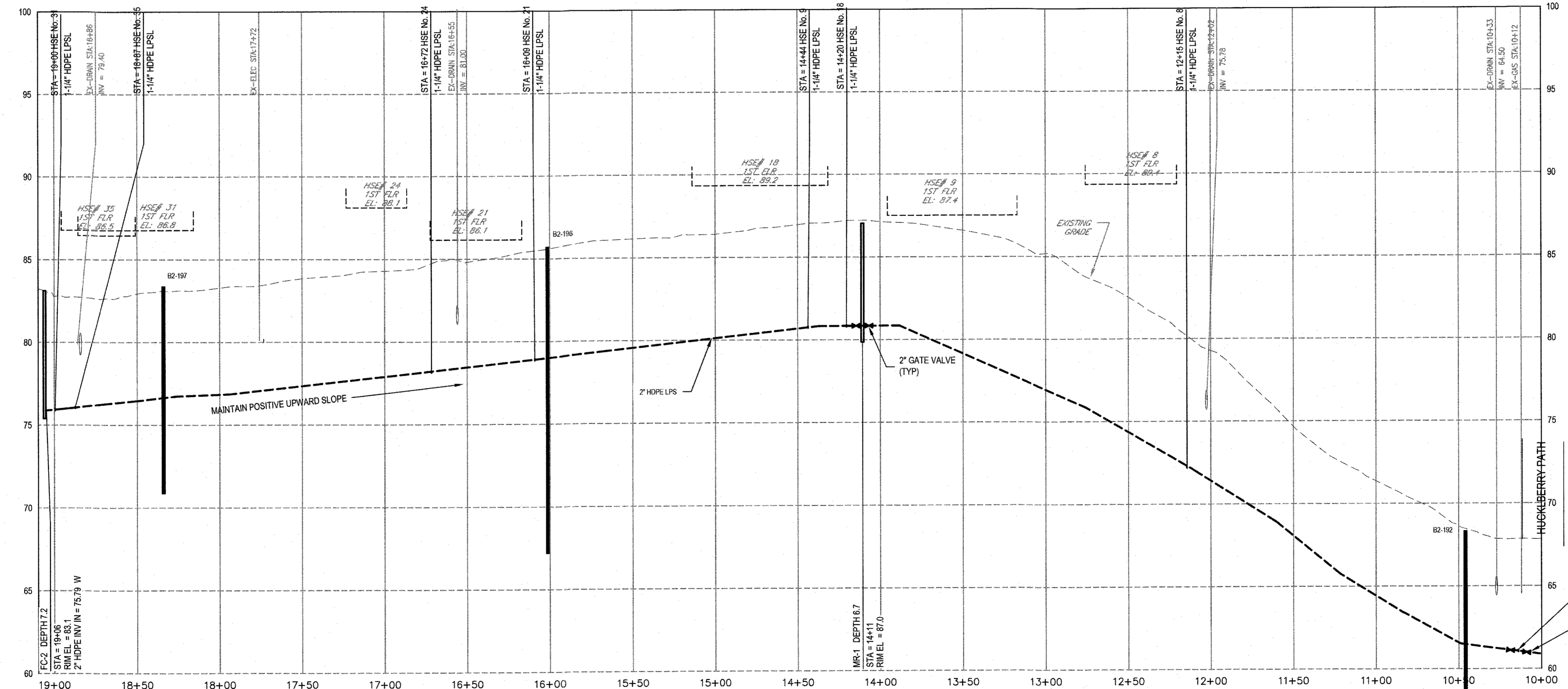
SADIES WAY - PROFILE (BID ALTERNATE #3)
