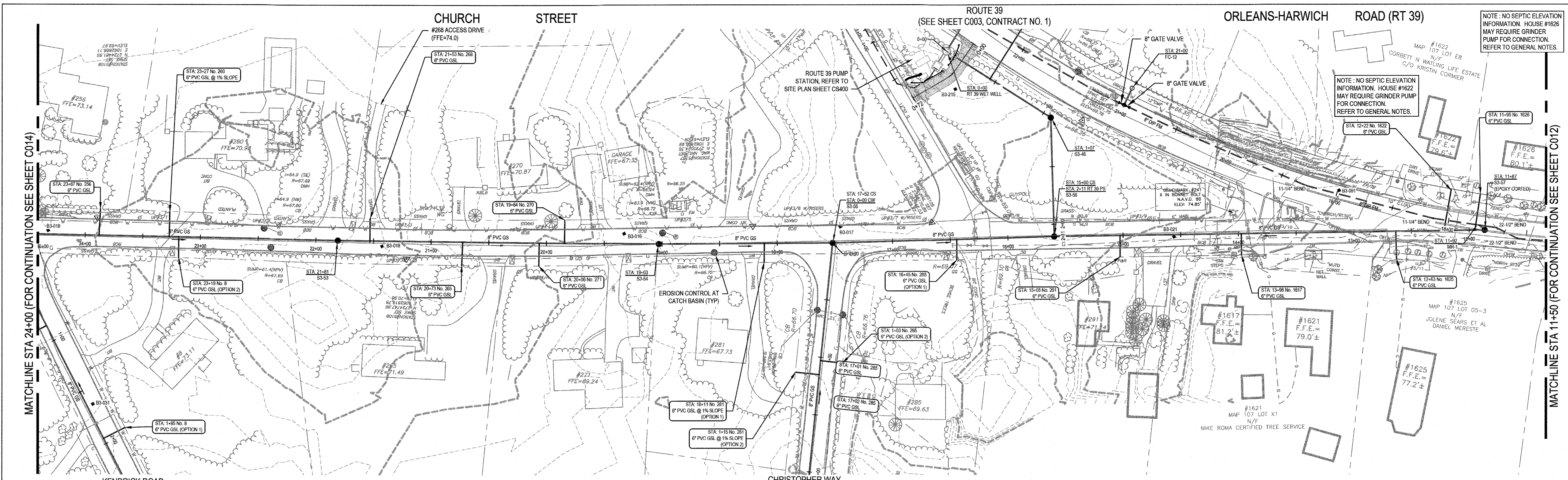
CHURCH STREET/ORLEANS-HARWICH ROAD - PLAN 2 SCALE 1" = 40'
