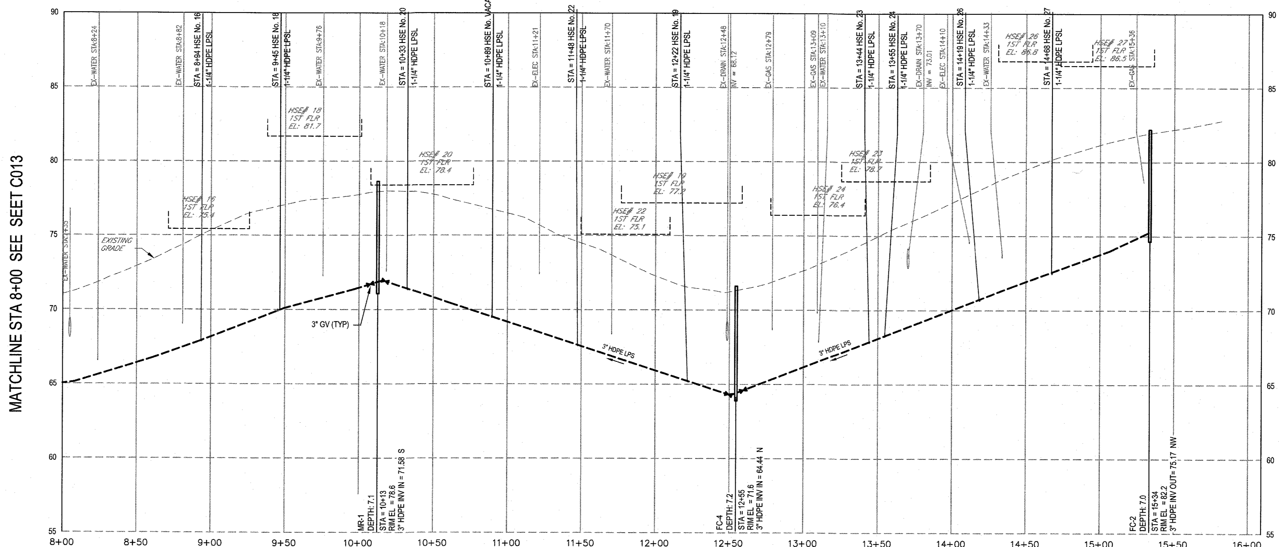
WALDEN WAY - PROFILE 2 (BID ALTERNATE #3)
