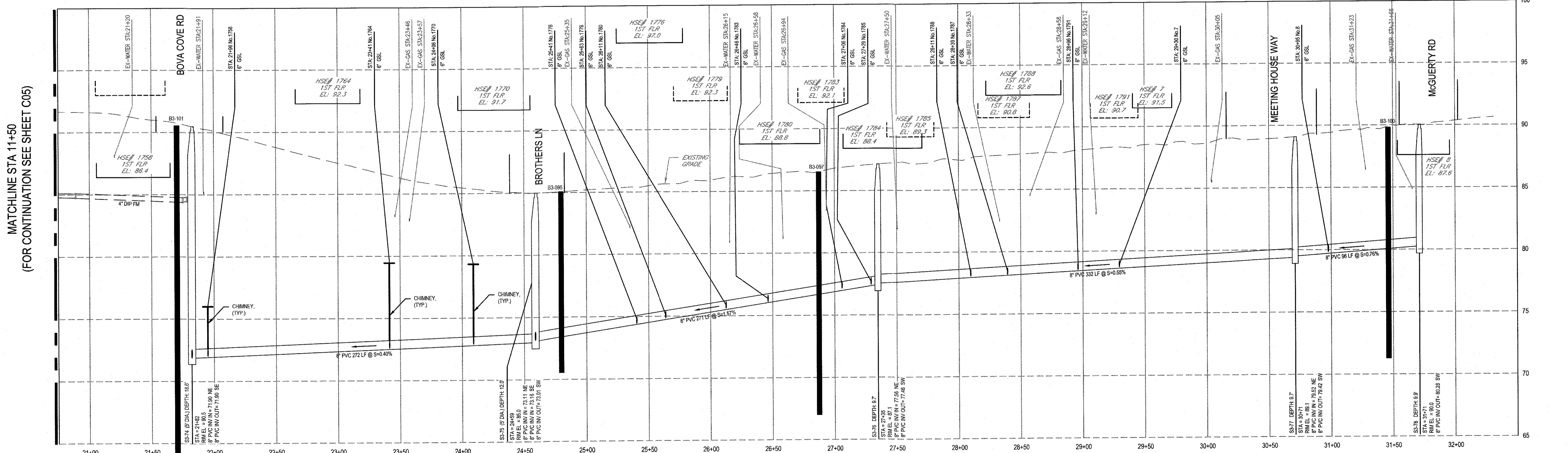
ORLEANS-HARWICH ROAD (ROUTE 39) - PROFILE 8 SCALE HORIZ 1" = 40' VERT 1" = 4'
