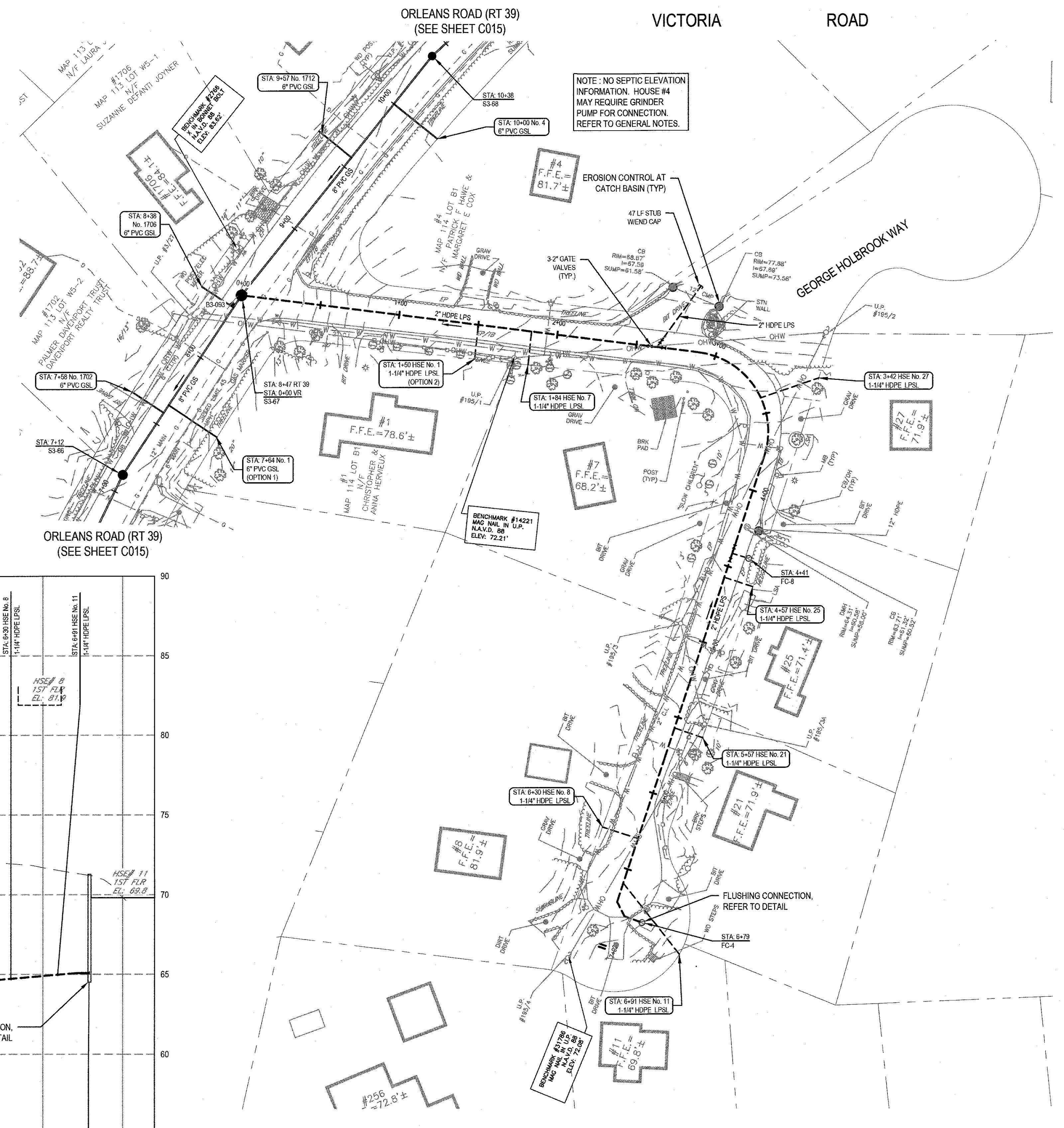
VICTORIA ROAD - PLAN (BID ALTERNATE #1) SCALE 1" = 40'
