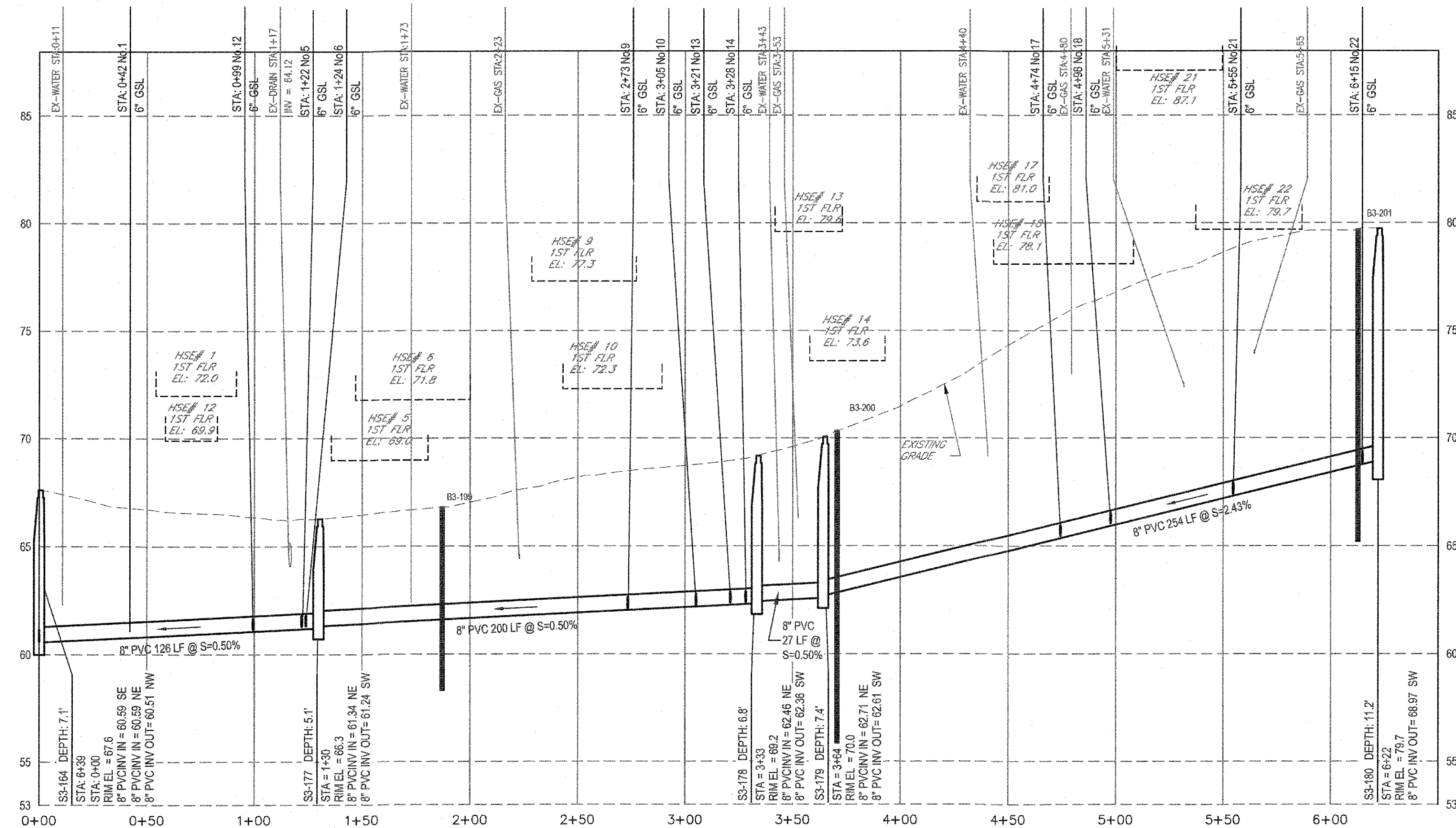
STEVENS WAY - PROFILE SCALE HORIZ 1" = 40' VERT 1" = 4'
