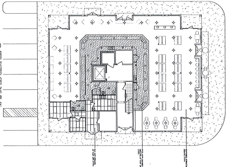
2 REFLECTED CEILING PLAN SCALE: AS SHOWN
