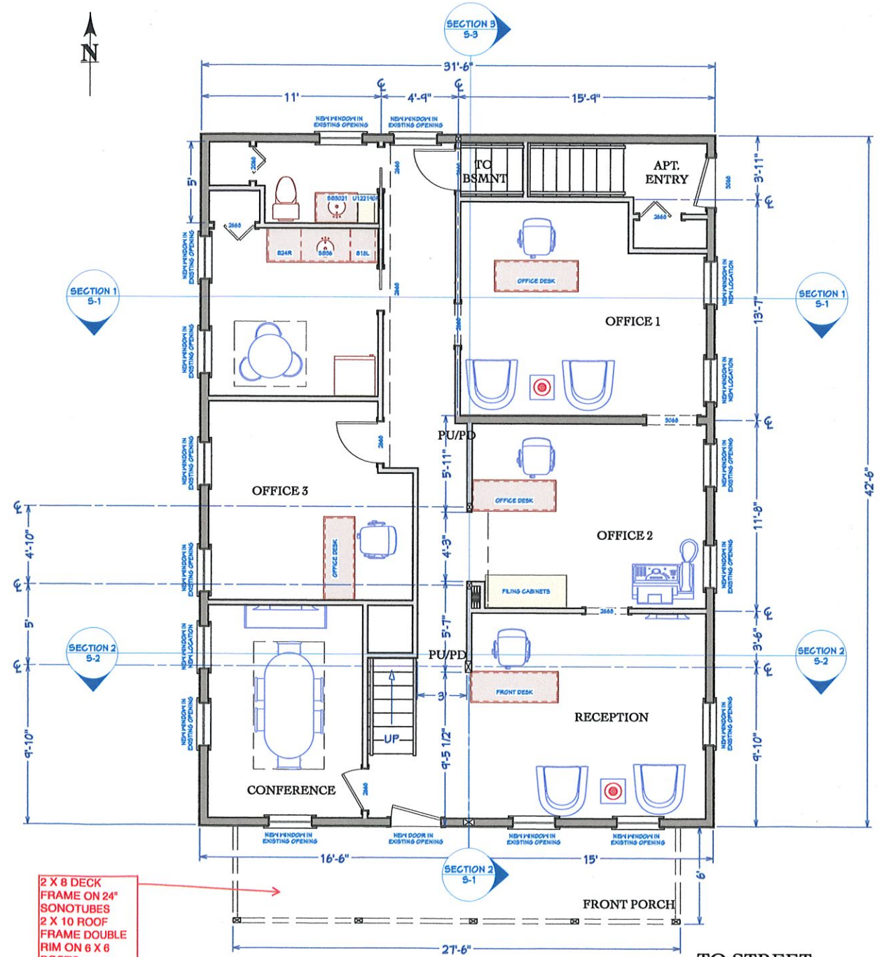
FIRST FLOOR PROPOSED
