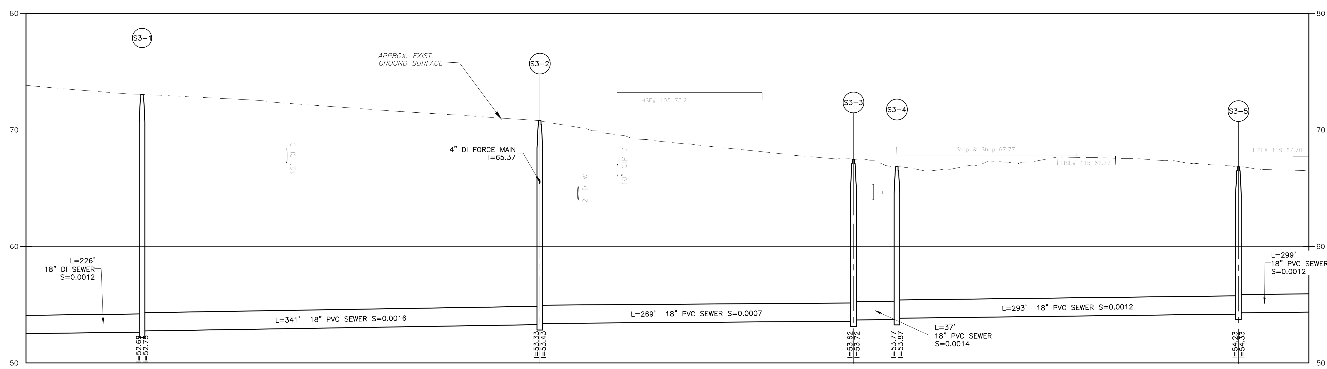
PROFILE SCALE: HORIZ. 1"=40'-0" VERT. 1"=4'-0"
