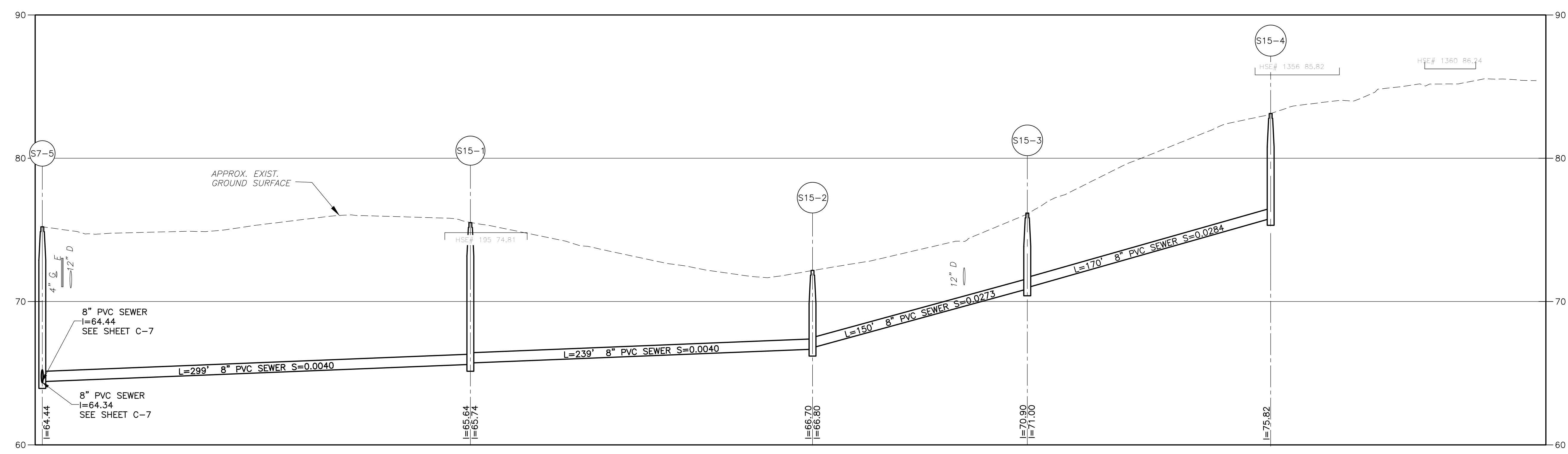
PROFILE SCALE: HORIZ. 1"=40'-0" VERT. 1"=4'-0"
