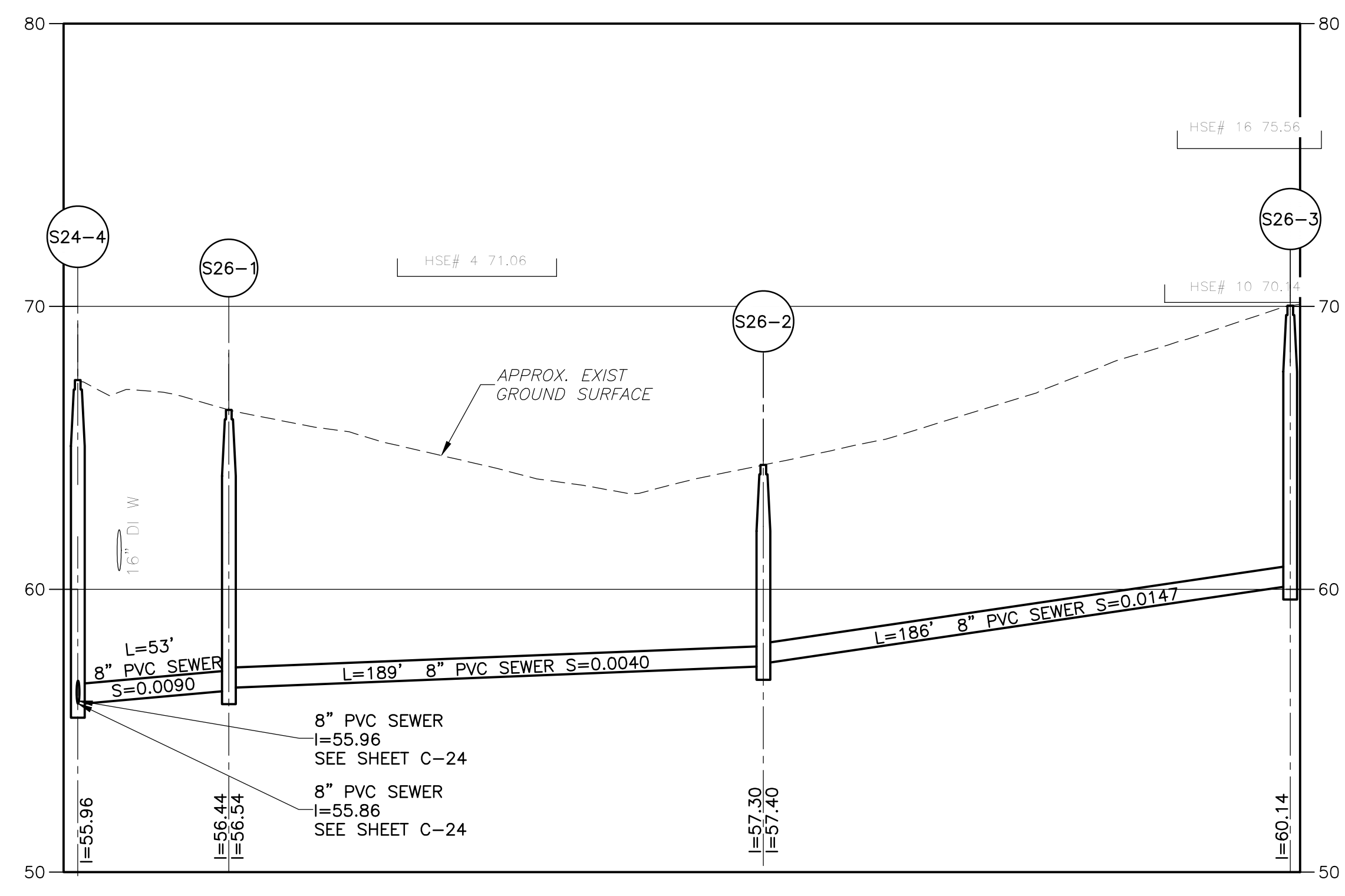
PROFILE SCALE HOR: 1"=40'-0" VERT: 1"=4'-0"
