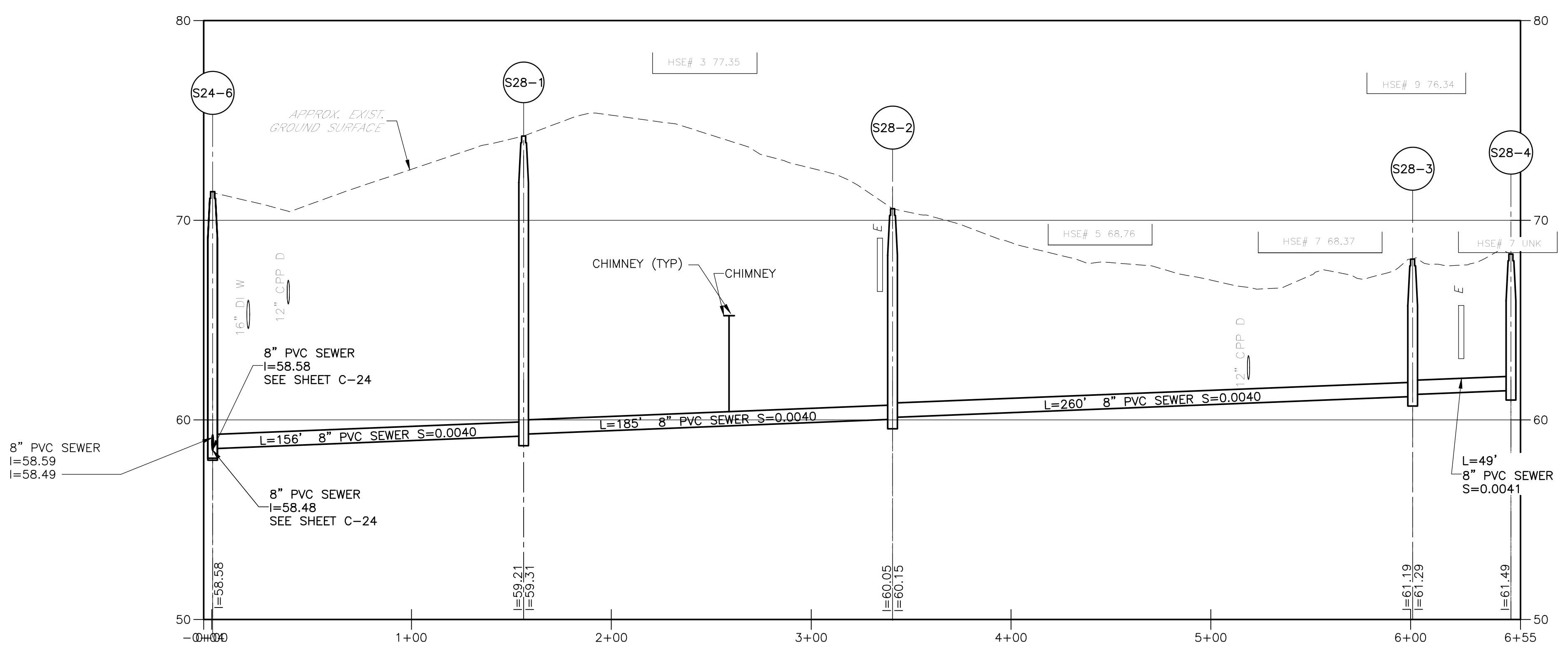
PROFILE SCALE HOR: 1"=40'-0" VERT: 1"=4'-0"
