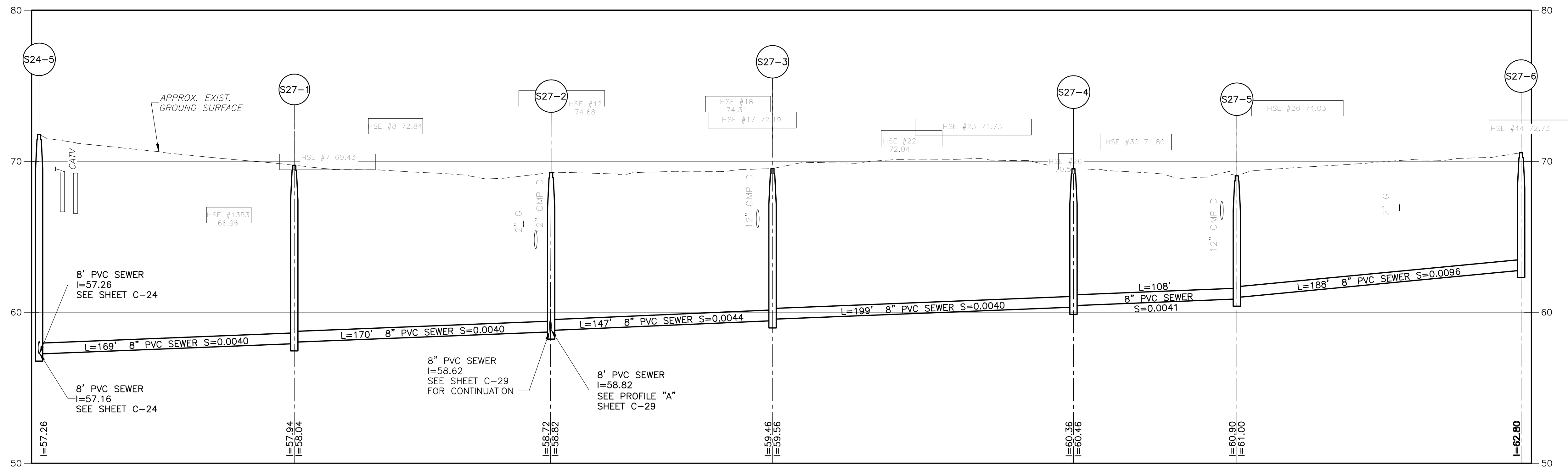
PROFILE SCALE HOR: 1"=40'-0" VERT: 1"=4'-0"
