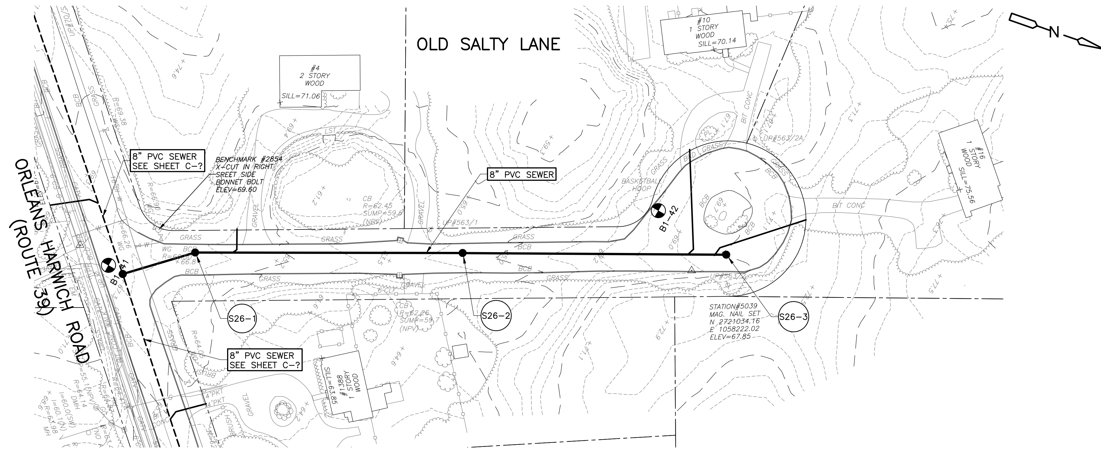
PLAN SCALE 1"=40'-0"
