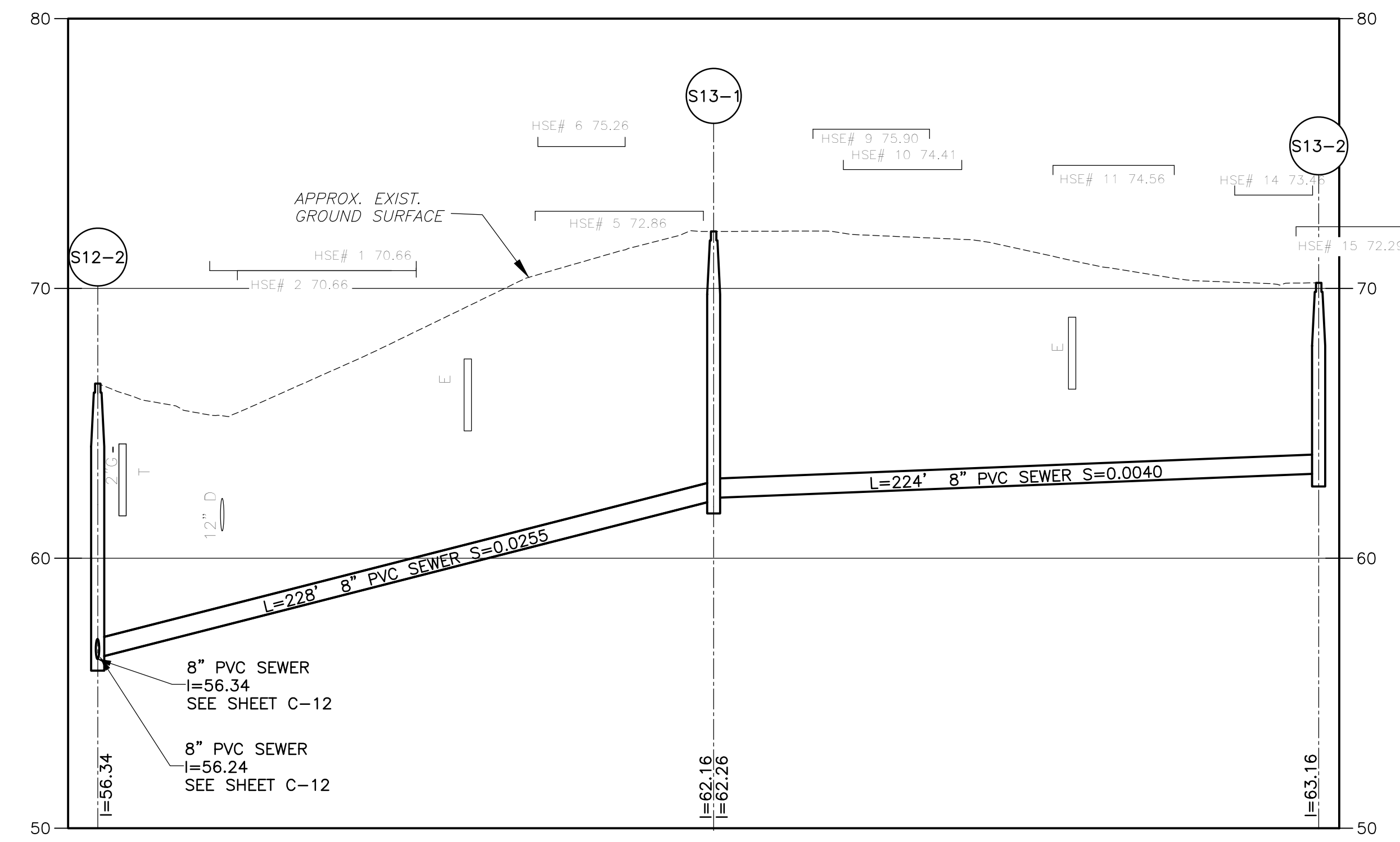
PROFILE SCALE: HORIZ. 1"=40'-0" VERT. 1"=4'-0"
