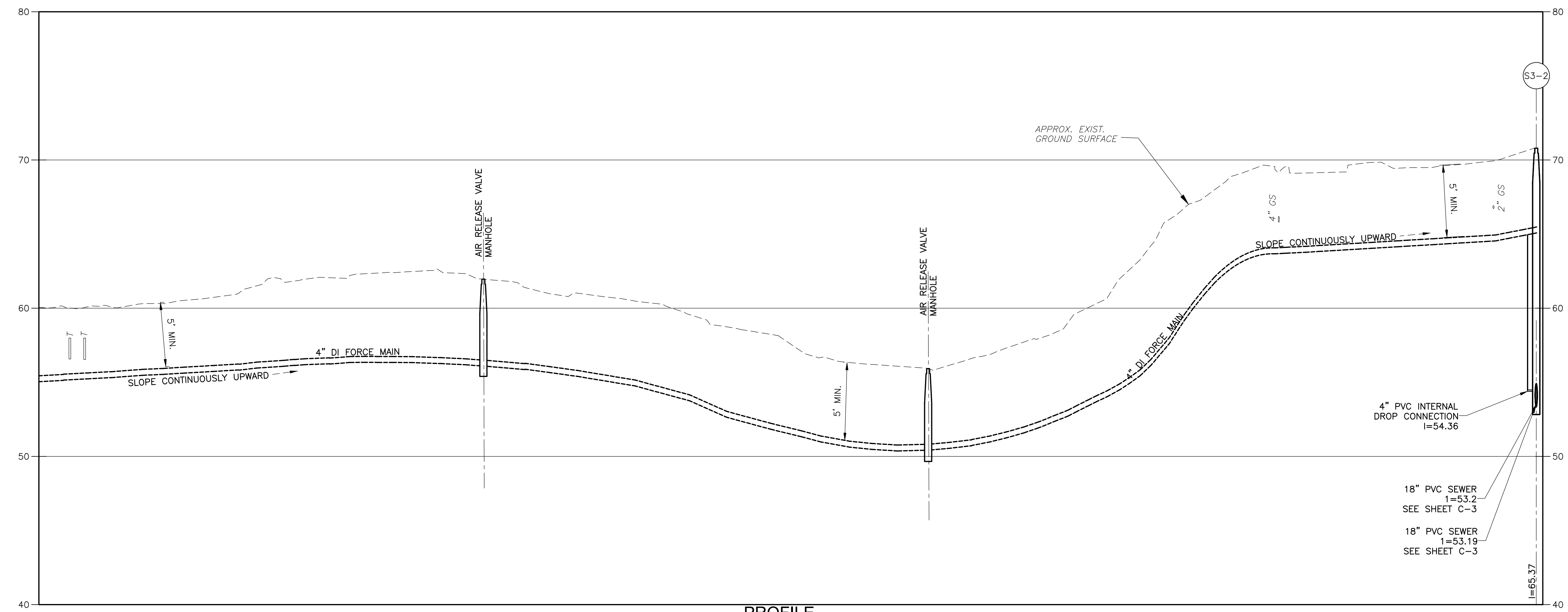
PROFILE SCALE: HORIZ. 1"=40'-0" VERT. 1"=4'-0"
